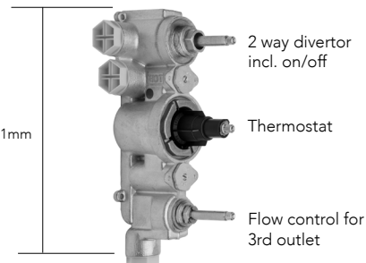
V132-IS Concealed thermostatic valve - rough Requires T1003. This valve has a two-way divertor plus an extra controlled outlet giving 3 options.
