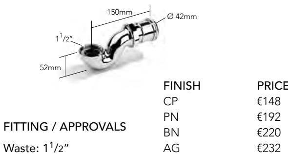
V195 Low P trap for freestanding bath
