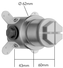
V168-IS Concealed 3-way divertor - rough Requires T1068.
