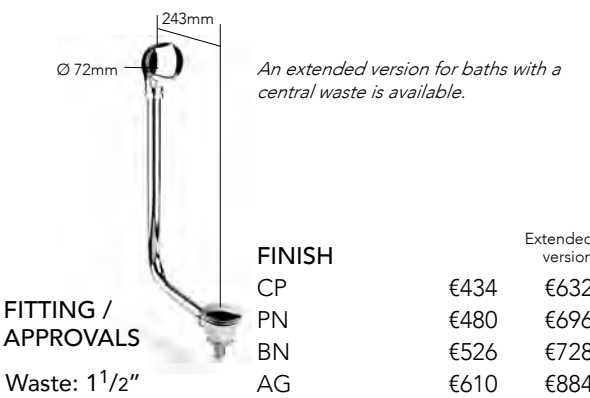
V197 Bath click-clack waste with overflow for freestanding baths
