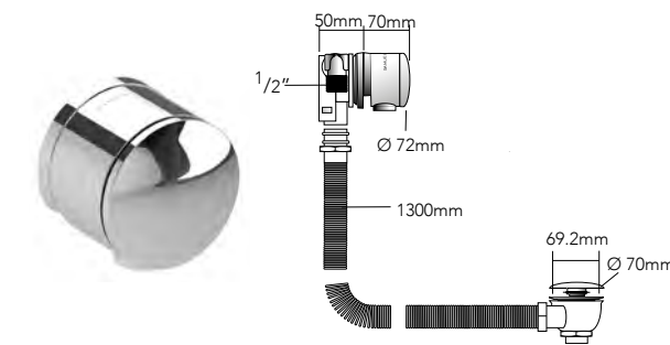
V145 Overflow filler (high pressure) with click waste
