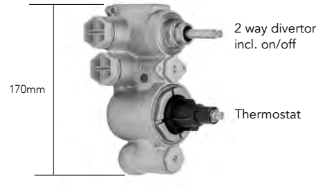
V111-IS Concealed thermostatic valve - rough Requires T1011. This valve has a 2-way diverter.
